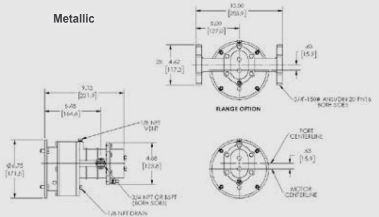
Metallic version includes bearing flush ports per drawing below
