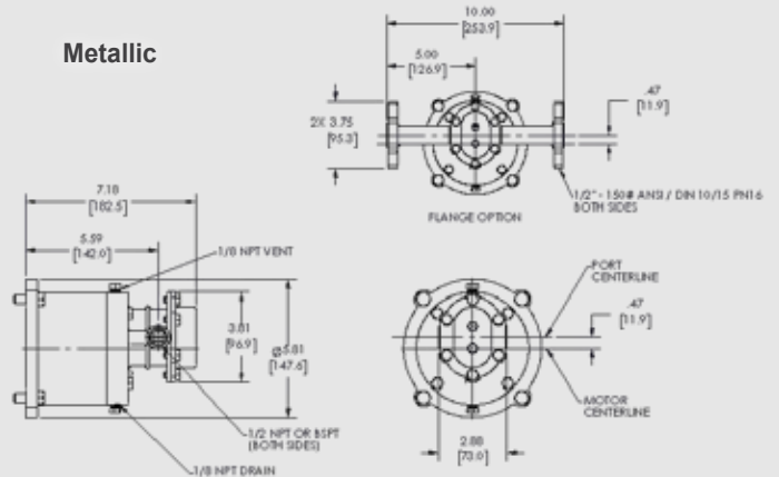
Metallic version includes bearing flush ports per drawing below
